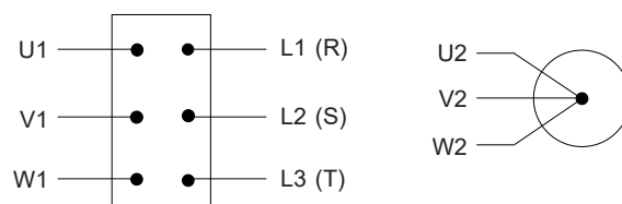
Panel connection
