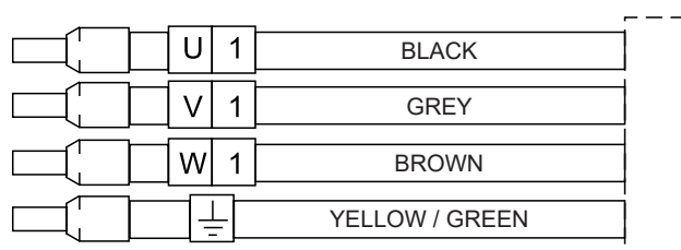
Electric pump cable conductor identification
