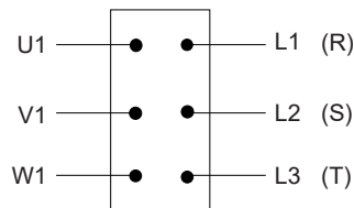
Panel connection
