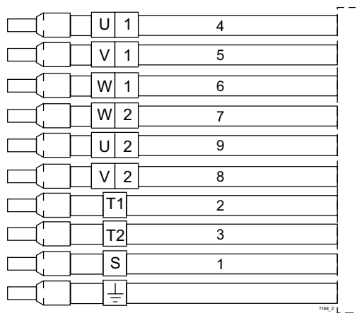
Electric pump cable conductor identification
